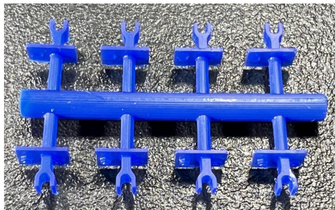
Above: Tube Brake Beam for older 8' passenger trucks. Below: CNW Short Queen Posts. Special castable resin and ready for direct burnout.
