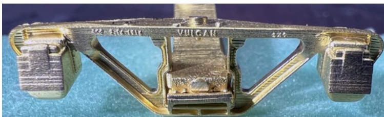
S scale Vulcan truck direct burnout from castable resin.
