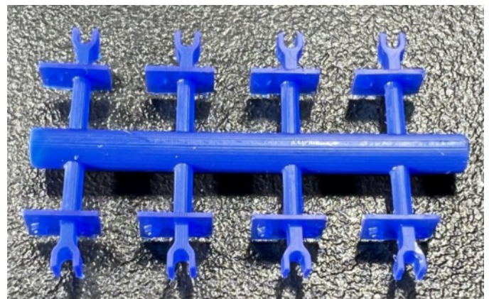
Above: Tube Brake Beam for older 8' passenger trucks. Below: CNW Short Queen Posts. Special castable resin and ready for direct burnout.
